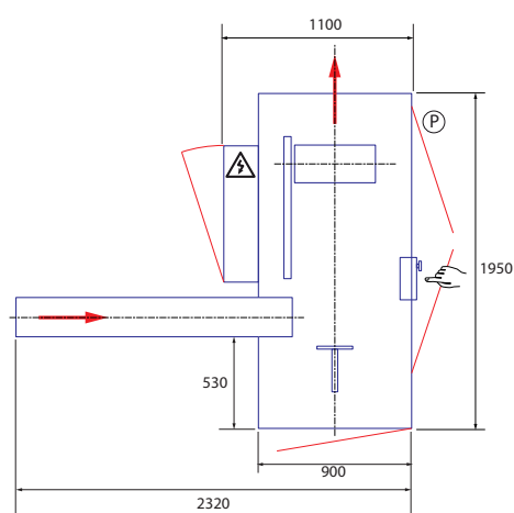
General dimensions of an HL configuration
